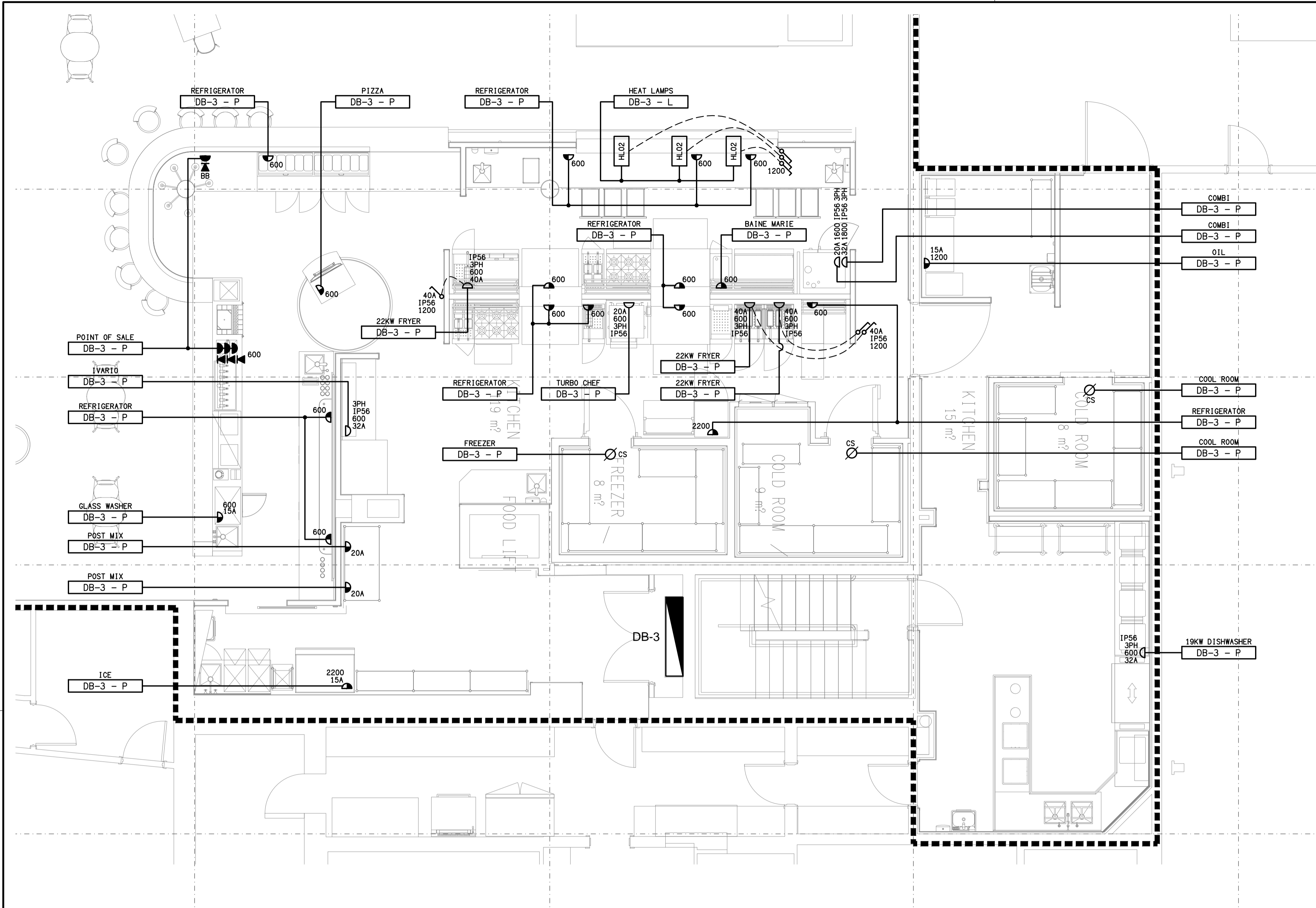
DETAIL B KITCHEN & BAR FLOOR PLAN SCALE 1:50
